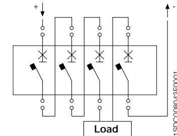
A) 3+1 poles in series (1000 Vdc)
