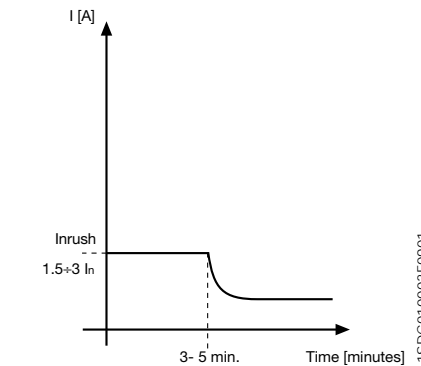
Inrush current diagram
